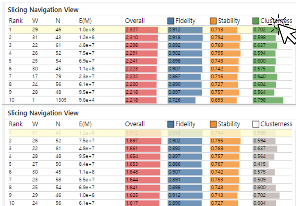
Fig. 5. The interaction technique for measure selection in Slicing Navigation View. Users can directly select which measure to use when calculating the overall score within three measures: Motif Fidelity , Motif Stability , and Motif Clusterness .
