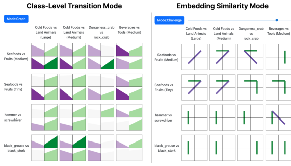
Figure 5: The example of Task Pair Comparison View with Embedding Similarity Mode (right) and Class-Level Transition Mode (left). The Embedding Similarity Mode shows the line patterns to reveal the task transition challenges, while the Class-Level Transition Mode simplifies the transition graph.
